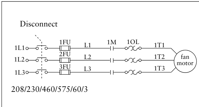
Motor Starter Wiring
