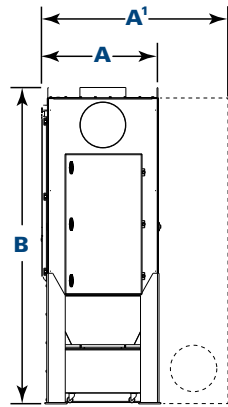
TG4 Front View
