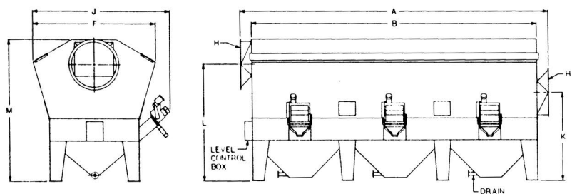
Model "MCD" (7000 cfm – 50,000 cfm)
